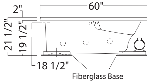
10-jet Bodywrap System SB-3660 BWS (illustrated)
