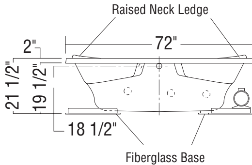
12-jet Bodywrap System SBHG-4272 / BWS (illustrated)
