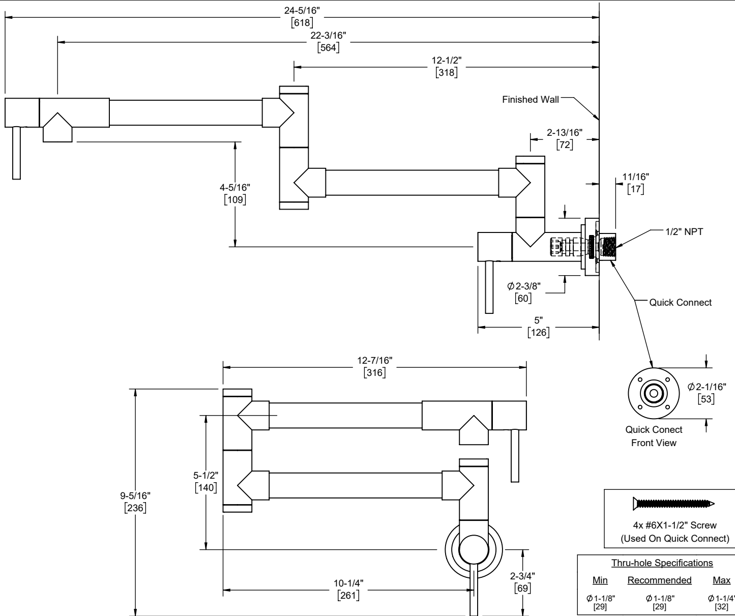
K50-200-ST shown
